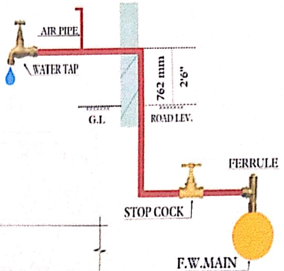
DETAILS OF FEEDING POINT
